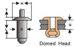
Domed Head
